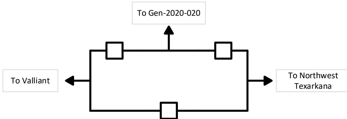
Figure 1: Point of Interconnection (POI INFORMATION) One-Line Diagram
